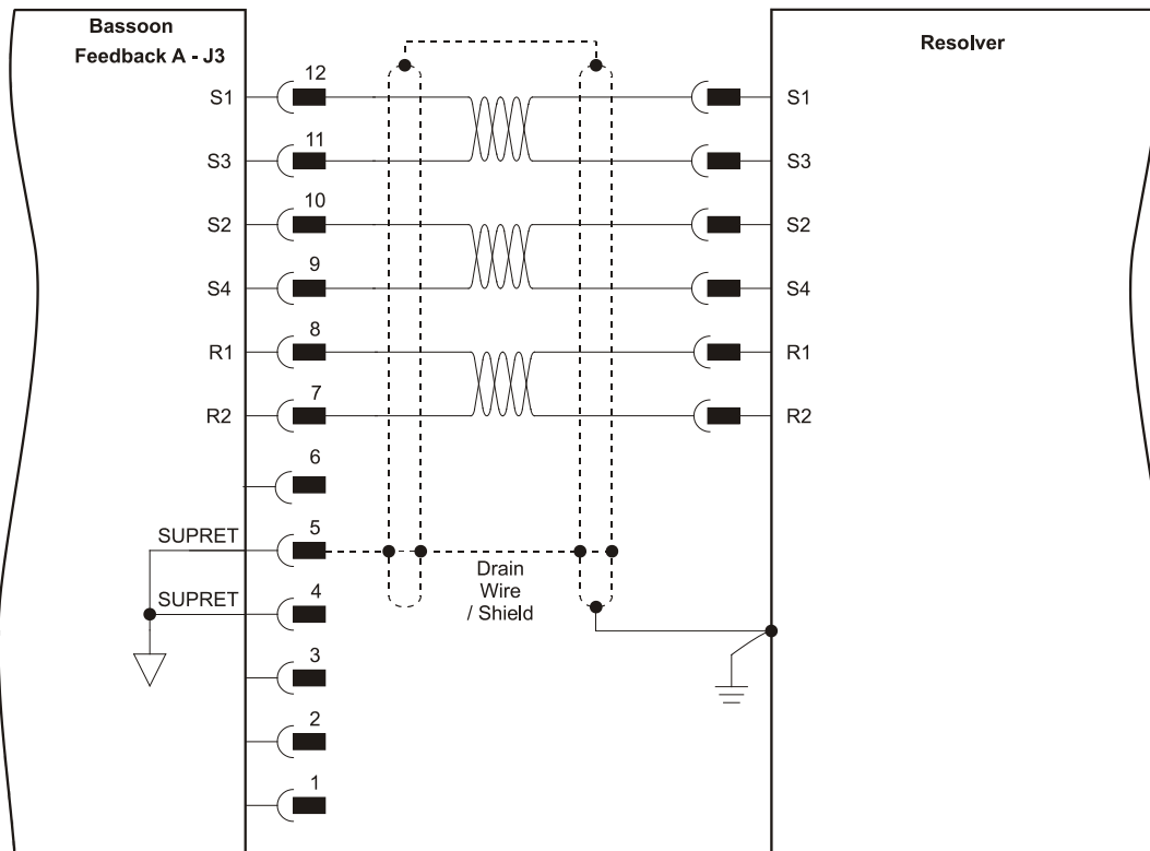
Figure 14: Main Feedback – Resolver Connection Diagram
