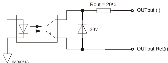
Figure 33: Digital Output Schematic
